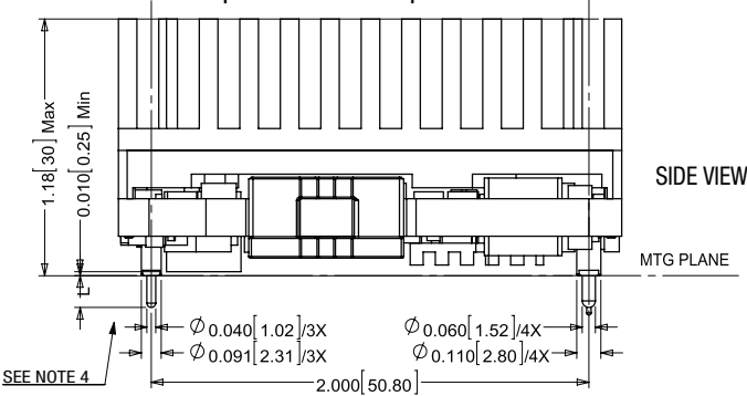
Baseplate+Heatsink Option*
