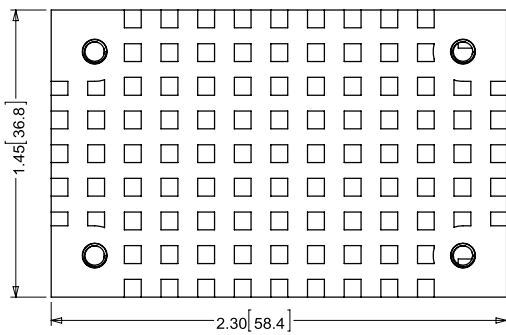
Baseplate+Heatsink Option*
