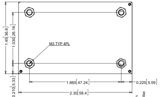
Baseplate Option
