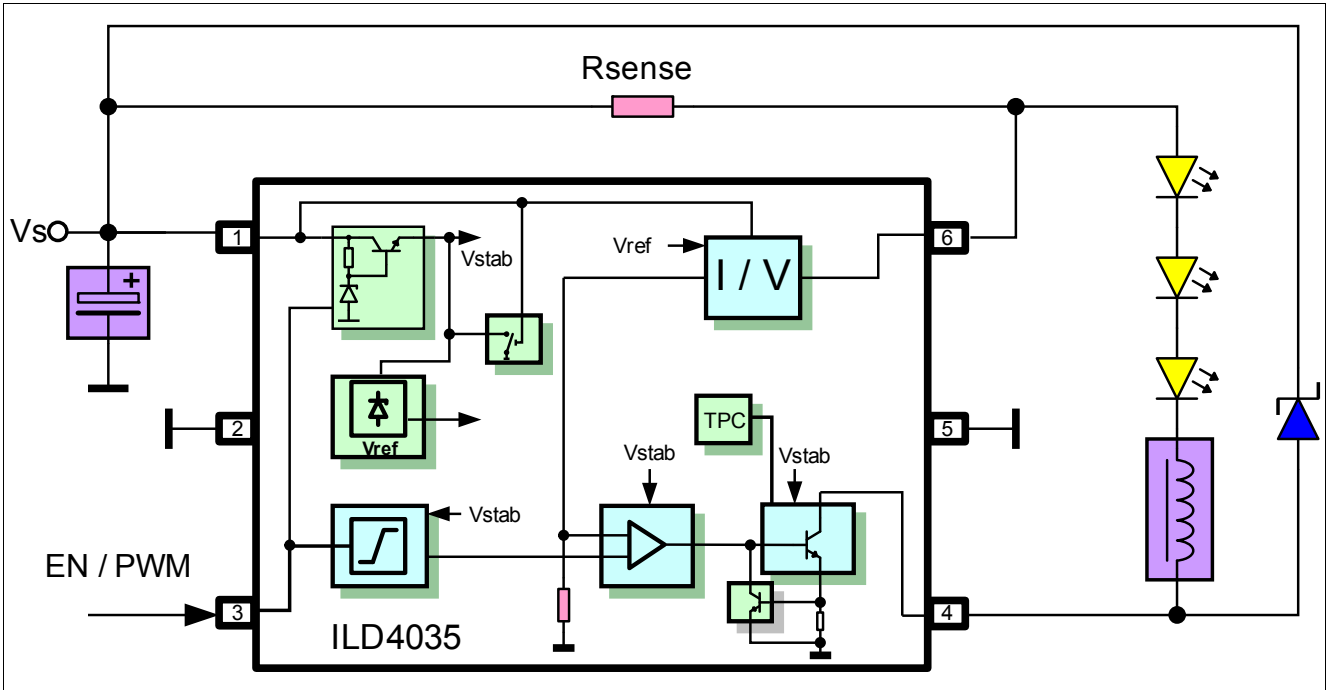
Figure 5 Application Circuit
