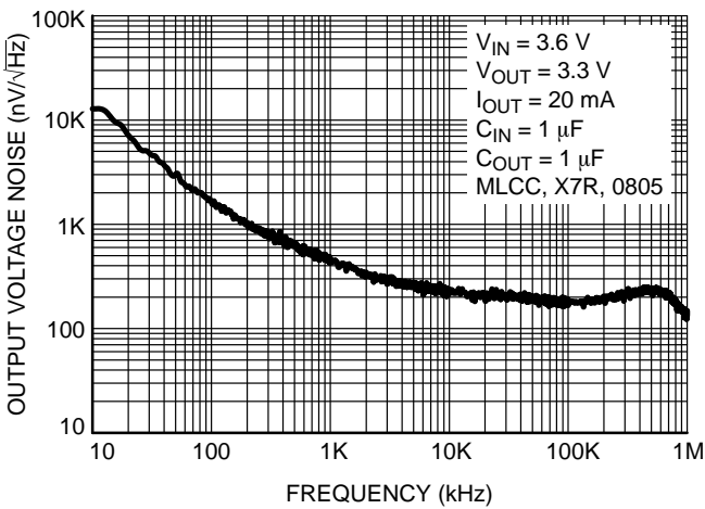
Figure 19. Output Voltage Noise Spectral Density for V_{OUT} = 3.3 V , I_{OUT} = 20 mA , C_{OUT} = 1 \mu F
