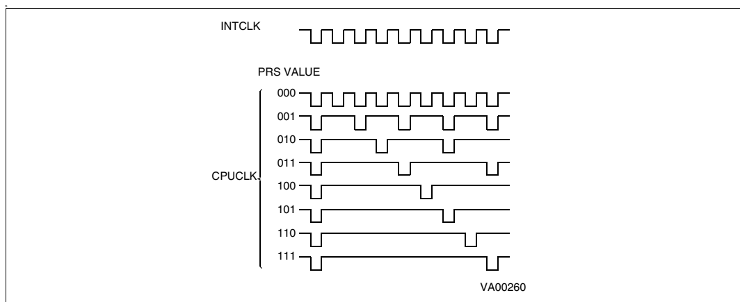
Figure 62. CPU clock prescaling
