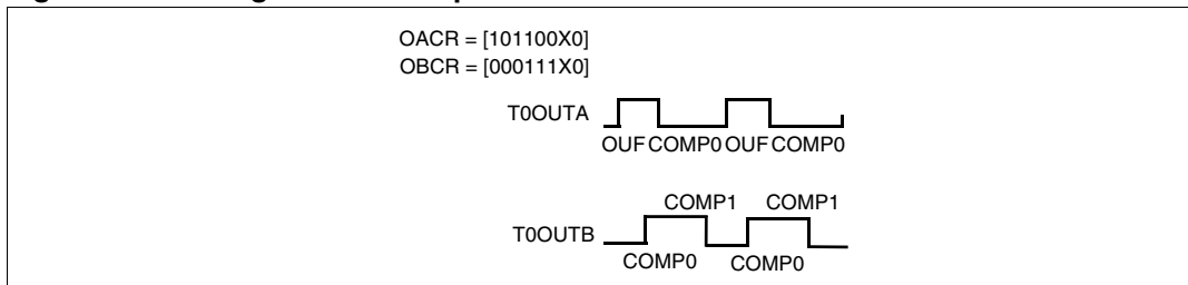
Figure 117. Configuration example 3
