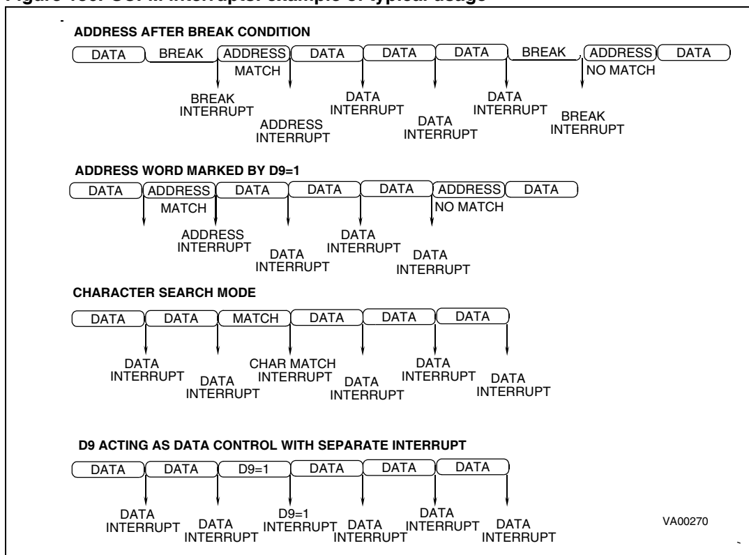
Figure 130. SCI-M interrupts: example of typical usage
