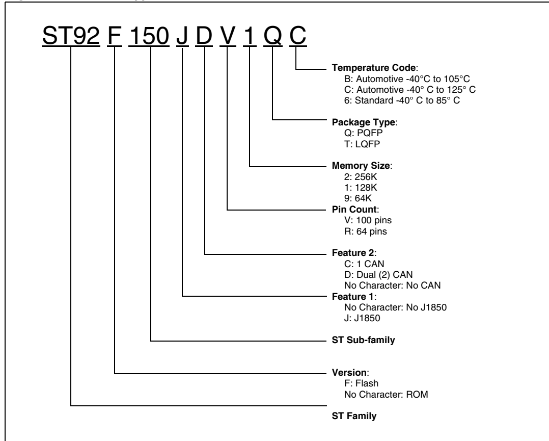
Figure 197. Device types
