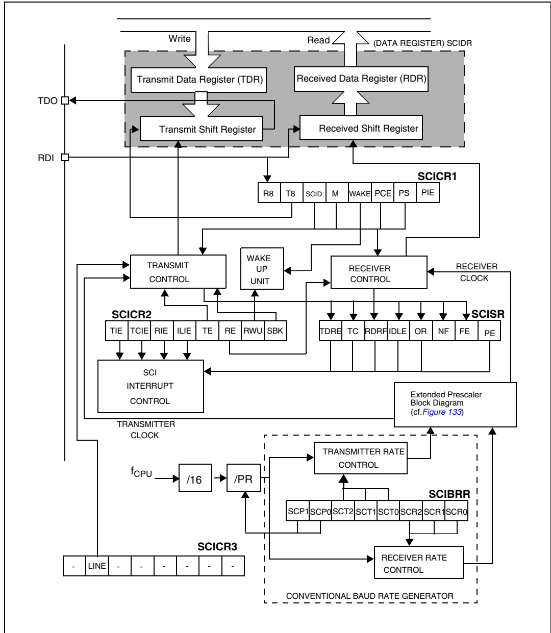
Figure 131. SCI-A block diagram
