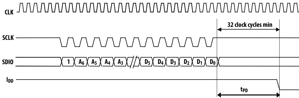
Figure 11: Power-down timing
