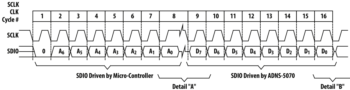
Figure 18. Read operation
