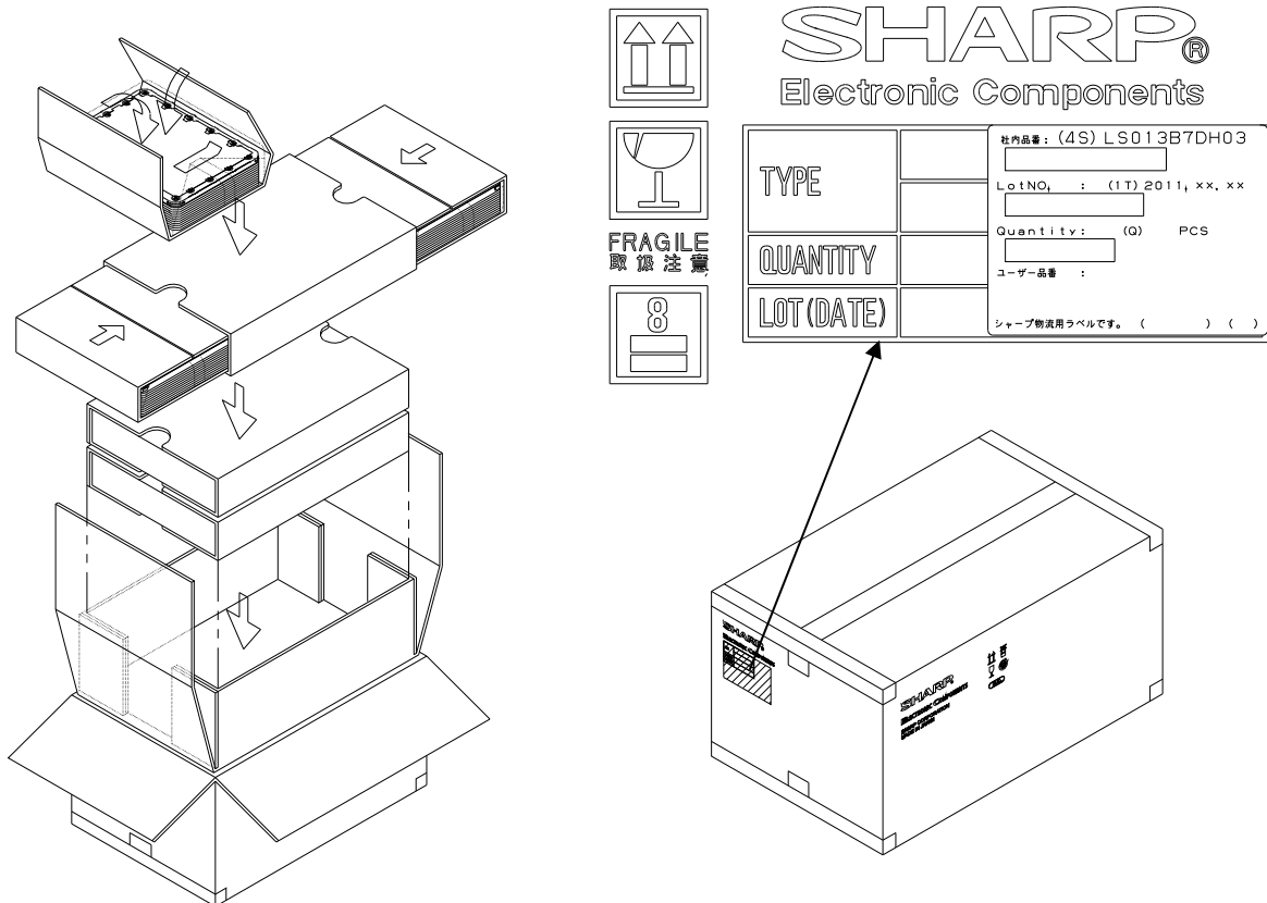
Figure 10-2: packing condition
