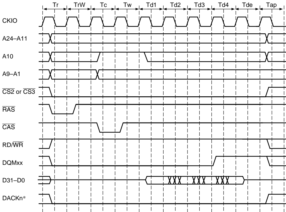
Figure 7.20 (a) Burst Read Wait Specification Timing (Auto-Precharge) Except t_{\text{Eye}}:t_{\text{Peye}} 1:1
