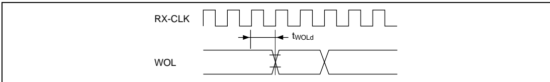
Figure 21.76 WOL Output Timing
